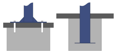
above ground installation
